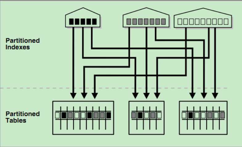
图 8-5 Global Partitioned Index
