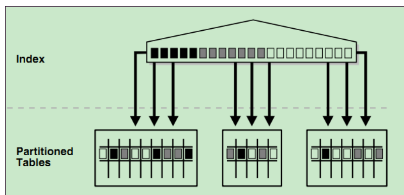
图 8-4 Global Non-Partitioned Index
